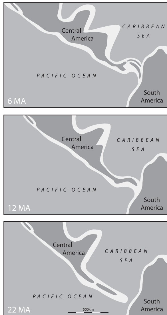
Fig. 1. Closure of the Isthmus of Panama. Palaeogeographic interpretations of land (dark grey), shallow seas (light grey) and deep seas (medium grey) in Central America at 22, 12 and 6 Ma. The position and form of the Central American volcanic arc is derived from Coates et al. (2003, 2004), Farris et al. (2011) and Montes et al. (2012a) and emergent land interpreted from evidence presented in Coates et al. (2003, 2004), Kirby et al. (2008) and O’Dea et al. (2012).
